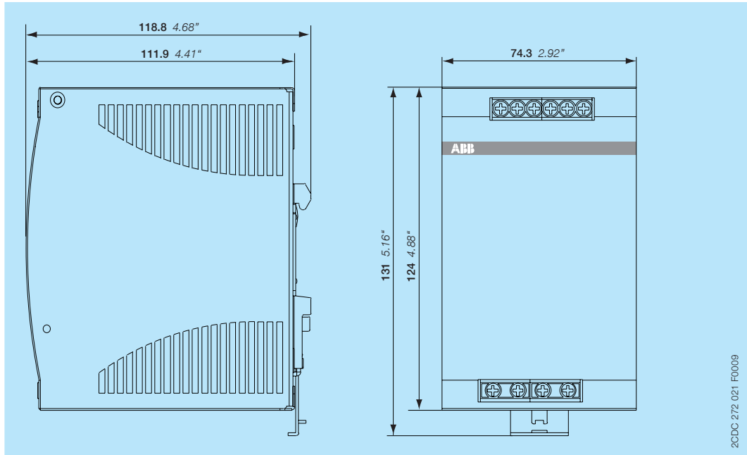
Power supply
