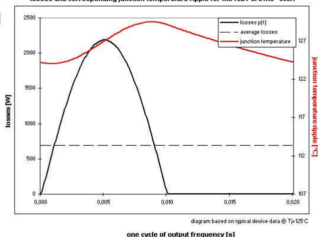
losses and corresponding junction temperature ripple for the IGBT at I_{rms} = 500 A
