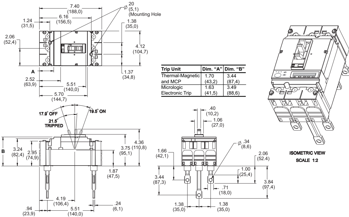
Figure 17: 15–150 A Rear Connected PowerPact H-Frame 3P Circuit Breaker
