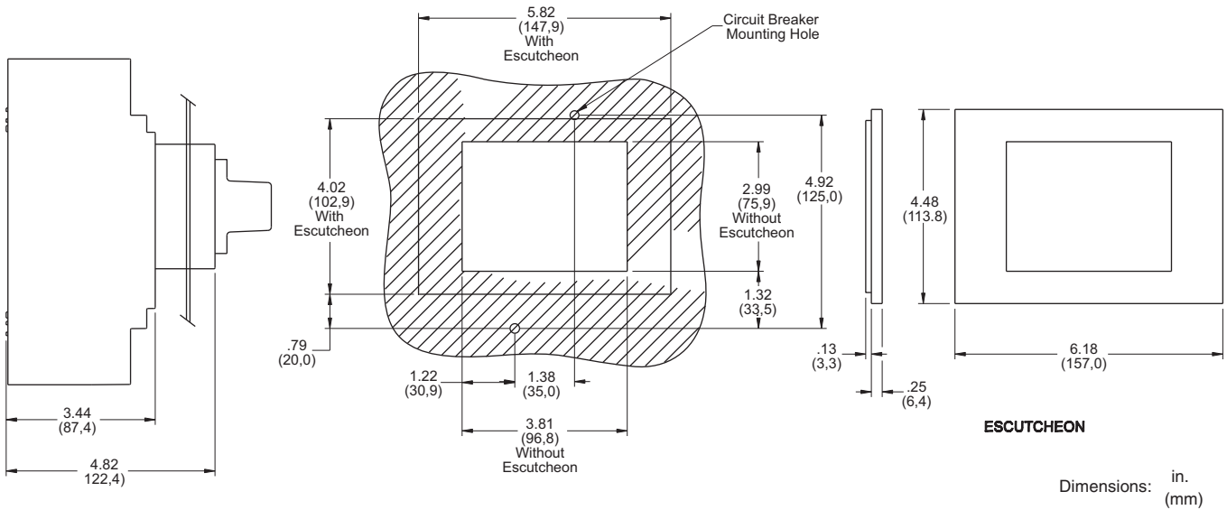
Figure 34: PowerPact H- and J-Frame Circuit Breaker Door Mounted Rotary Handle Cutout
