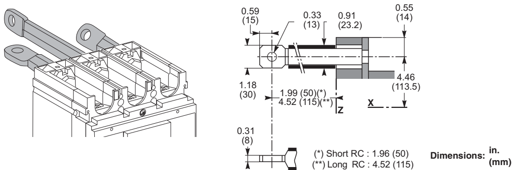
Figure 57: PowerPact L-Frame Circuit Breaker Rear Connections
