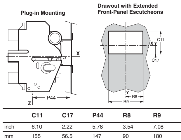
Figure 44: PowerPact L-Frame Circuit Breaker Front-Panel Cutouts
