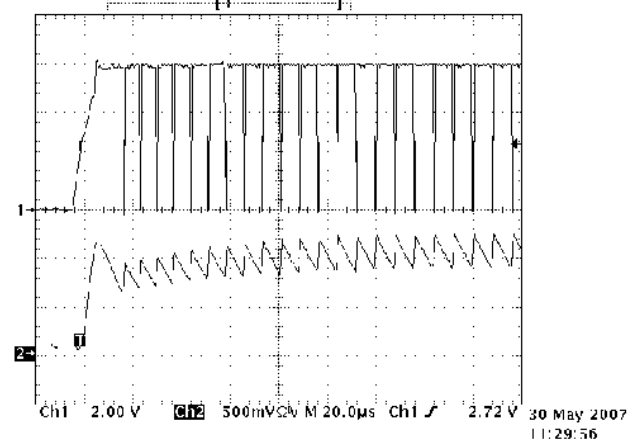
V_{IN} = 24V , R_S = 0.1\Omega , L = 68\mu H , 22nF on ADJ Soft-start operation. Output current (Ch2) and LX voltage (Ch1) Tek 5102 Single Seq 2.50 MS/s
