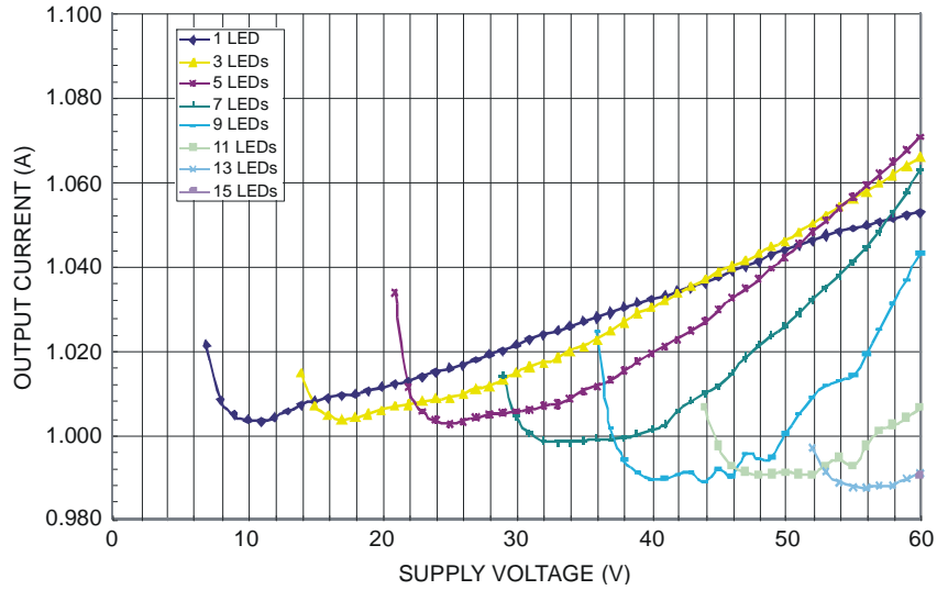
Output Current, L = 68μH
