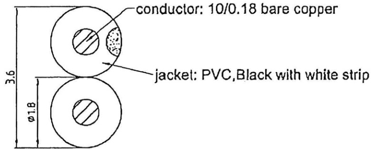
Cable Construction
