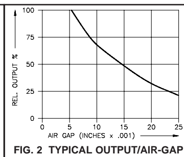
FIG. 2 TYPICAL OUTPUT/AIR-GAP
