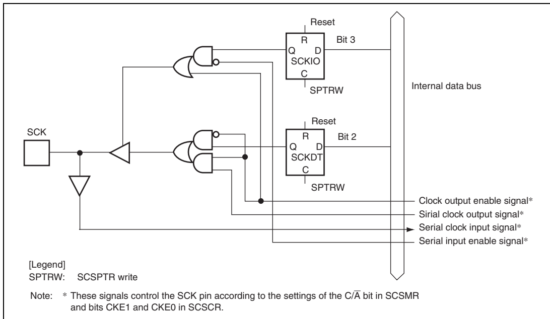
Figure 16.21 SCKIO Bit, SCK DT bit, and SCK Pin
