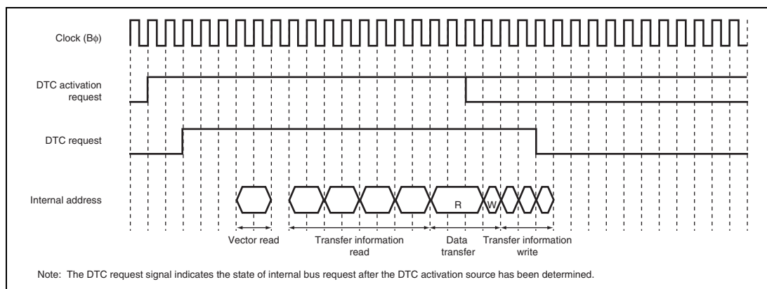
Figure 8.14 Example of DTC Operation Timing: Normal or Repeat Transfer with DTPR = 1 (Activated by On-Chip Peripheral Module; Iφ: Bφ: Pφ = 1: 1/2: 1/2; Data Transferred from On-Chip Peripheral Module to On-Chip RAM; Transfer Information Is Written in 3 Cycles)
