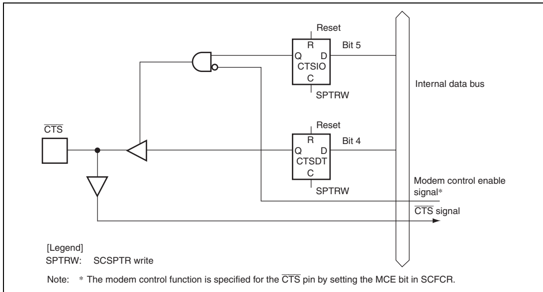
Figure 16.20 CTSIO Bit, CTS DT bit, and \overline{\text{CTS}} Pin
