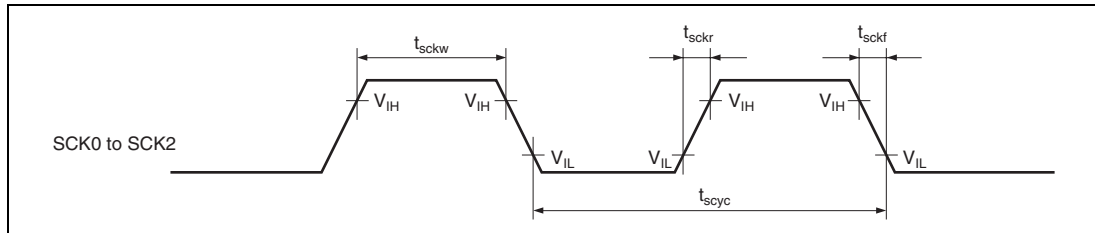
Figure 24.21 Input Clock Timing
