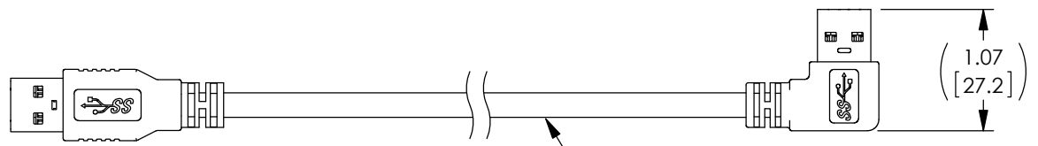
UL STYLE 20276, (2) TWISTED PAIR, 30AWG WITH ALUM/POLY FOIL SHIELD AND DRAIN WIRE, (1) UNSHIELDED TWISTED PAIR, 30AWG, (2) CONDUCTORS, 24AWG, OVERALL ALUMINUM/MYLAR AND BRAIDED SHIELD, JACKET: PVC, BLUE (PANTONE 300C) (NOM DIA. .217" [5.5], MIN BEND RAD 2.17" [55])
