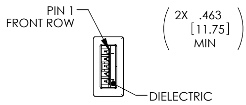
"P1" USB 3.0 SERIES "A" PLUG CONTACTS 30μ GOLD
