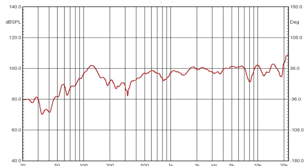
CH A dB SPL 1/6 Octave 48kHz 16K Rectangular Start 0.00ms Stop 341.31ms FreqLO 2.93Hz Length 341.31ms
