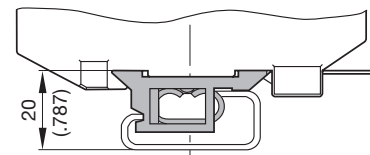
9102100000 TS32 adapter
