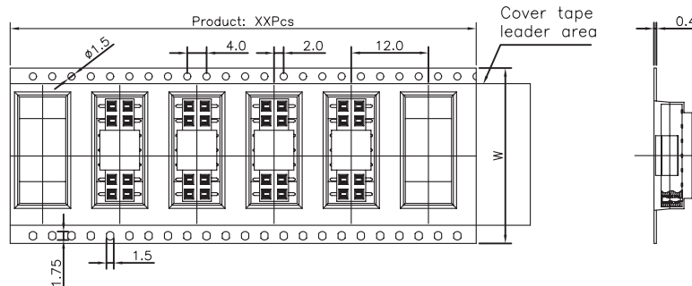
For Reel width (dimension W)32,44mm ,Double row hole
