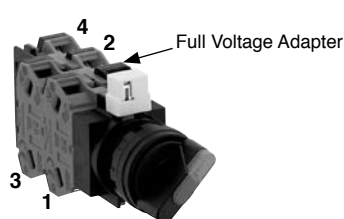
Illuminated Selector (Full Voltage Type)
