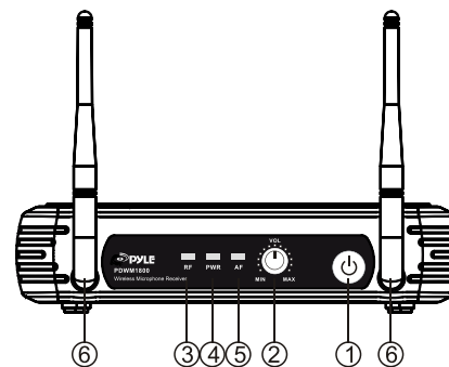
Front Panel
