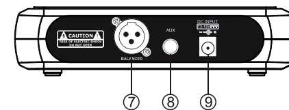
Rear Panel
