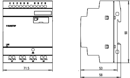
Base Module (without Display)
