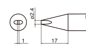
T33-D6 Shape 6D
