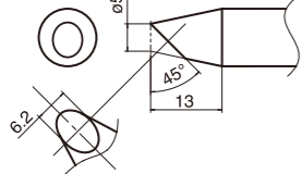
T33-D32 Shape 3.2D
