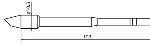
T33-BC3 Shape 3BC
