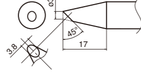
T33-BC6 Shape 6BC
