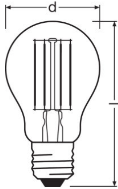
P RF CLAS A 75 8 W/827 E27, P CLAS A 75 8 W/840 E27
