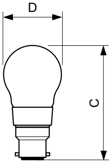
filament 4.5W-40W 470lm NAD 2700K B22D
