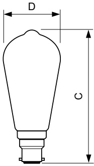
filament 7W-60W 806lm NAD 2700K B22D
