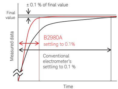
20 pA range settling time 2 V step, 100 GΩ, 1 PLC
