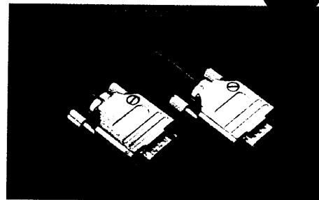
9 pole D sub male to male wired using 2 pair individually screened low capacitance cable. Industry standard for remotes and machine control. The low capacitance cable allows long lengths to be run without problems.
