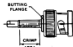
CRIMP AREA
