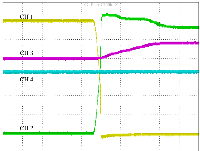
Figure 4: Oring for one feed loss (500µS/div): CH1: IinA (1A/div) CH2: IinB (1A/div). CH3: VRTN_OUT reference to -48V_OUT (10V/div). CH4: 3.3V (1V/div).
