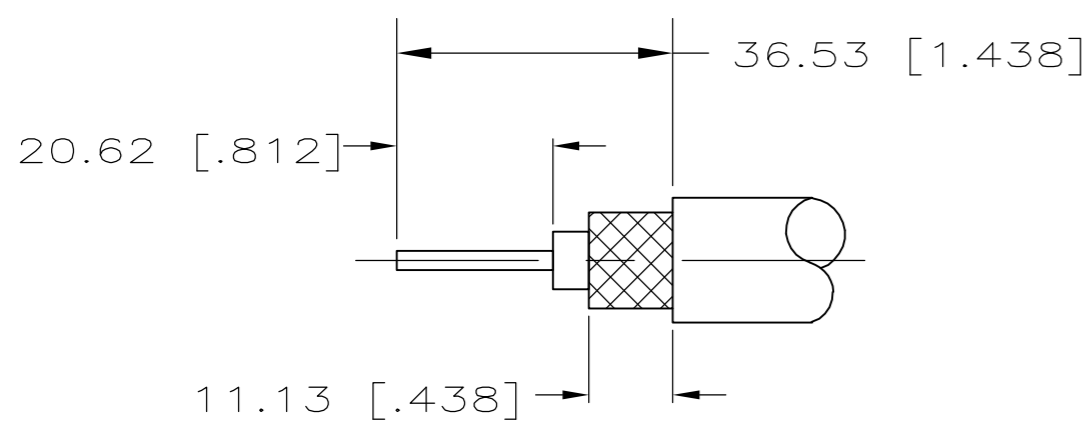
DETAIL A
