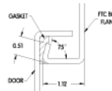
Rear View (Cross Section)
