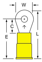
MVU10-6R Stud Size: 6 Wire Range: 12-10
