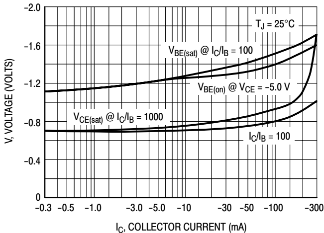
Figure 2. "ON" Voltage
