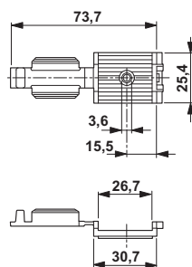
Dimensional drawing
