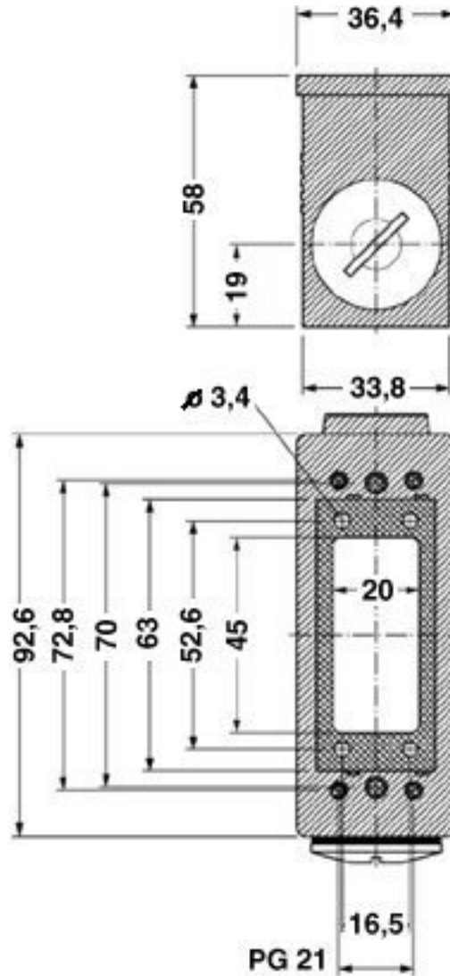
Dimensional drawing
