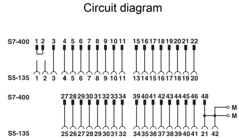
Connection scheme: FLKM S135/S400/SO121
