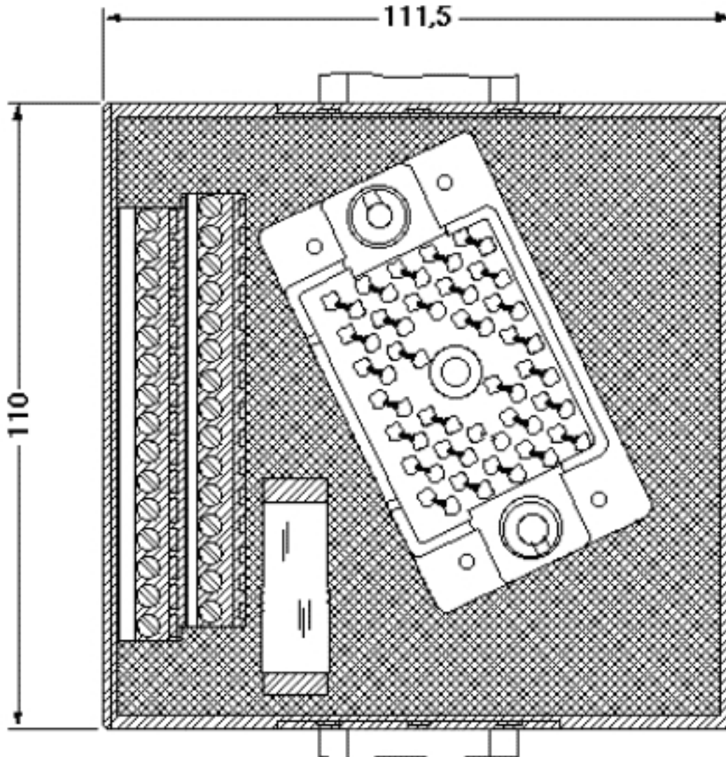
Dimensional drawing
