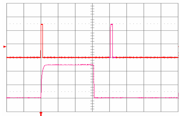
Fig. 16: Load current (top trace, 10 A/div., 50 ms/div.) into a 10 m\Omega short circuit during restart, at V_{in} = 48 V. Bottom trace (10 A/div., 2 ms/div.) is an expansion of the on-time portion of the top trace.
