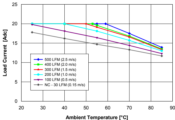
Fig. 2: Available load current vs. ambient air temperature and airflow rates for converter with G height pins mounted horizontally with air flowing from pin 1 to pin 3 and maximum FET temperature \leq 120^\circ\text{C} , V_{in} = 48\text{ V} .
