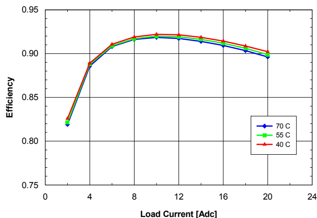
Fig. 4: Efficiency vs. load current and ambient temperature for converter mounted vertically with V_{in} = 48\text{ V} and air flowing from pin 1 to pin 3 at a rate of 200 LFM (1.0 m/s).
