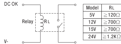
(c) Relay
