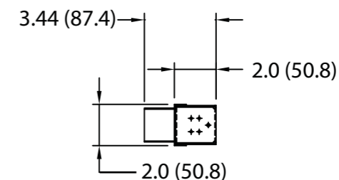
3 METER INLET POWER CORD
