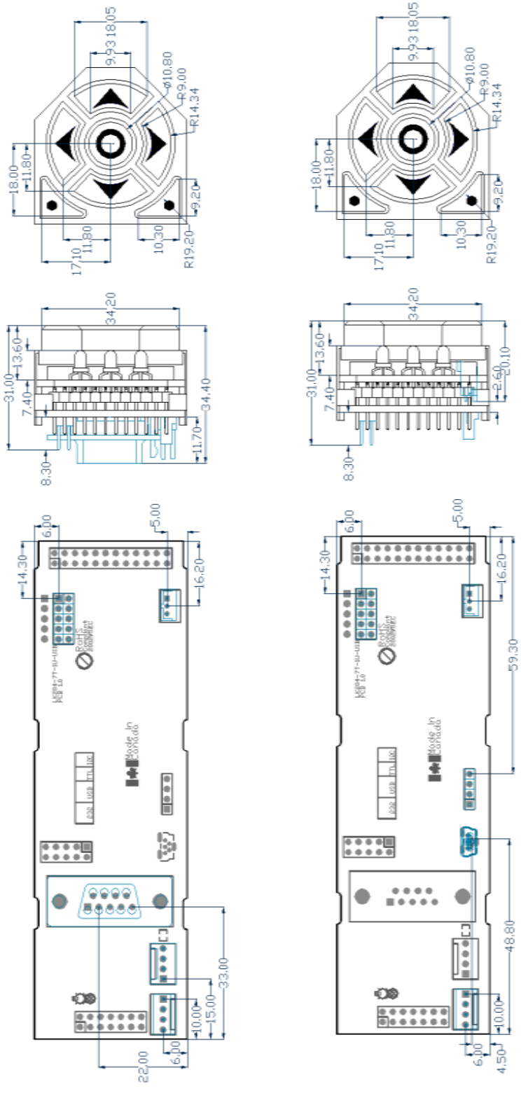
Figure 19: USB Model Drawing
