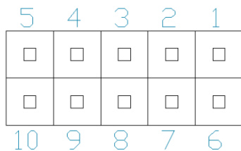
Figure 12: GPO Header
