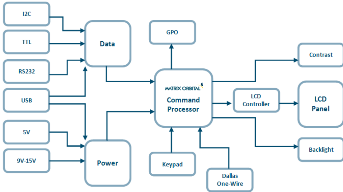
Figure 17: Functional Diagram
