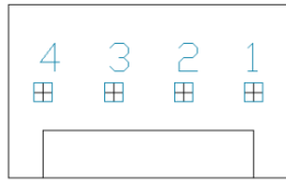
Figure 8: Communication/Power Header
