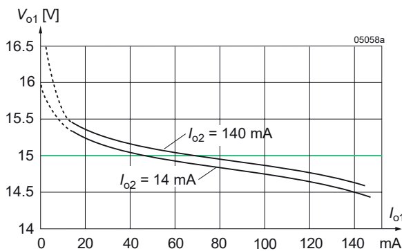
Fig. 11 Cross load regulation V_{o1} versus I_{o1} (typ.) for various I_{o2} (2 x 12 V)
