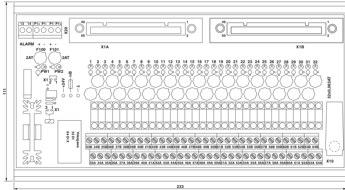
Dimensional drawing
