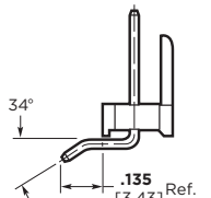
Retentive Leg
