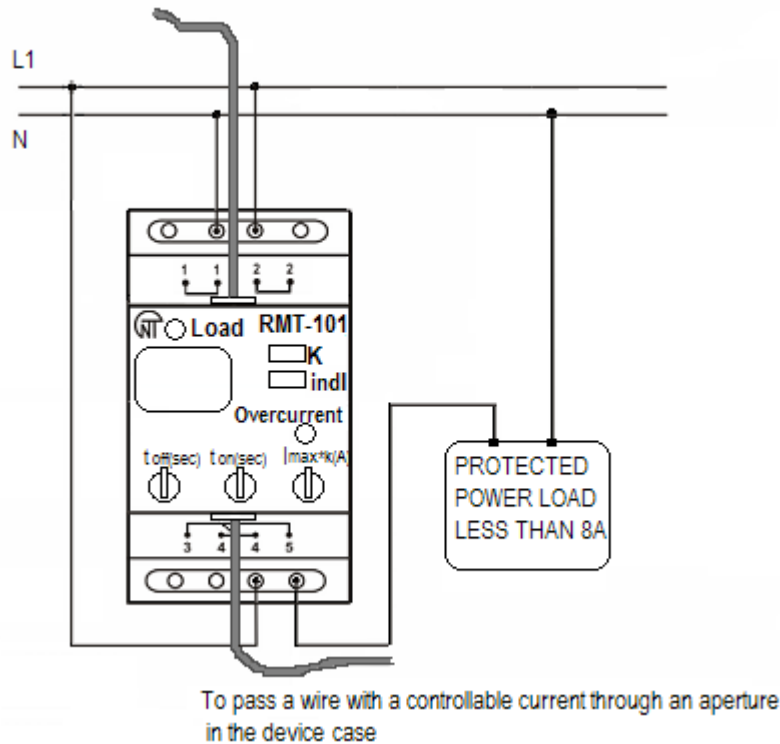
Figure 2 - Wiring diagram
