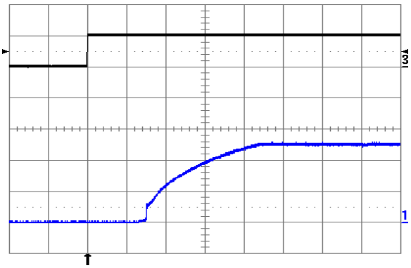
Fig. 2.5V.10: Turn-on transient at full rated load current (resistive) plus 10,000 µF at Vin = 24V, triggered via ON/OFF pin. Top trace: ON/OFF signal (5 V/div.). Bottom trace: output voltage (1 V/div.). Time scale: 1 ms/div.
