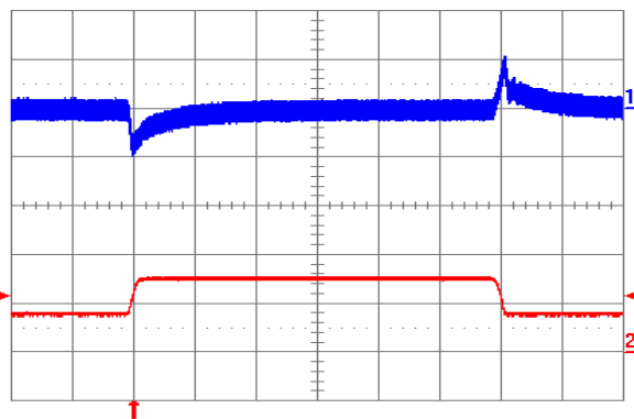
Fig. 2.5V.11: Output voltage response to load current step-change (3.75 A – 7.5 A – 3.75 A) at Vin = 24V. Top trace: output voltage (100 mV/div.). Bottom trace: load current (5 A/div.). Current slew rate: 0.1 A/µs. Co = 1 µF ceramic. Time scale: 0.2 ms/div.
