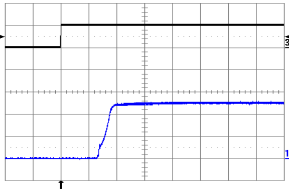
Fig. 2.5V.9: Turn-on transient at full rated load current (resistive) with no output capacitor at Vin = 24V, triggered via ON/OFF pin. Top trace: ON/OFF signal (5 V/div.). Bottom trace: output voltage (1 V/div.). Time scale: 1 ms/div.
