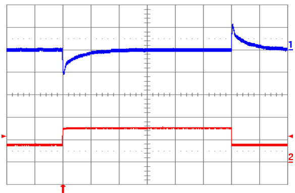
Fig. 2.5V.12: Output voltage response to load current step-change (3.75 A – 7.5 A – 3.75 A) at Vin = 24V. Top trace: output voltage (100 mV/div.). Bottom trace: load current (5 A/div.). Current slew rate: 5 A/µs. Co = 450 µF tantalum + 1 µF ceramic. Time scale: 0.2 ms/div.
