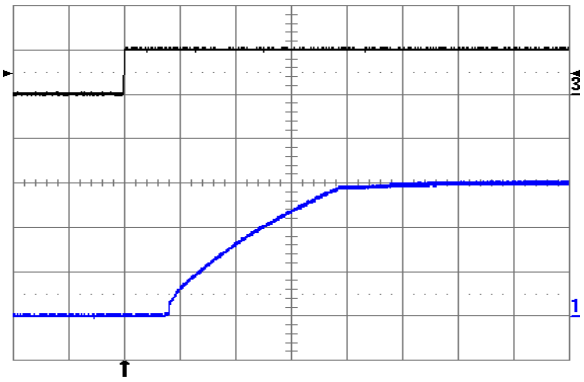
Fig. 6.0V.10: Turn-on transient at full rated load current (resistive) plus 10,000\mu\text{F} at V_{in} = 24\text{V} , triggered via ON/OFF pin. Top trace: ON/OFF signal (5 V/div.). Bottom trace: output voltage (2 V/div.). Time scale: 2 ms/div.
