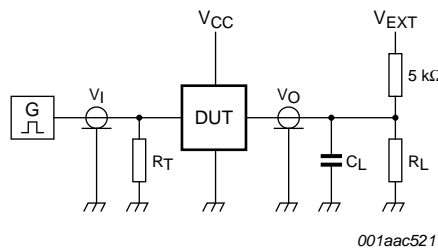
Test data is given in Table 10. Definitions for test circuit: R_L = Load resistance. C_L = Load capacitance including jig and probe capacitance. R_T = Termination resistance should be equal to the output impedance Z_o of the pulse generator. V_{EXT} = External voltage for measuring switching times.
