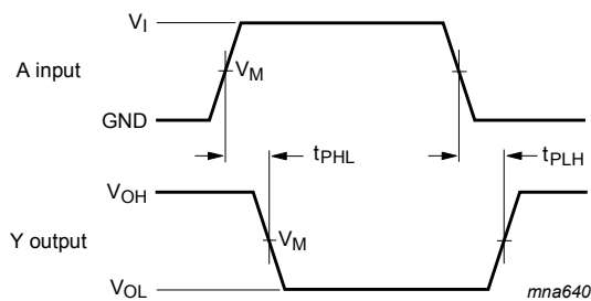
Figure 7. The input A to output Y propagation delays
