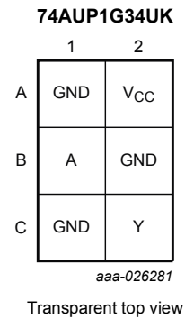
Figure 9. Ball mapping for SOT1454-1 (WLCSP6)
