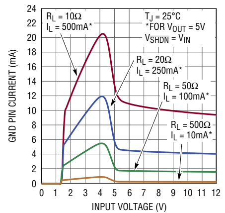
LT3065-5 GND Pin Current
