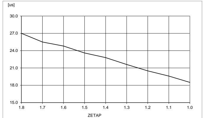
V_I=12\text{ V} , V_O=1.2\text{ V} , C_O = 3 \times 100\ \mu\text{F} + 270\ \mu\text{F}/10\text{m}\Omega , load step 3-9-3 A, 1 A/us.
