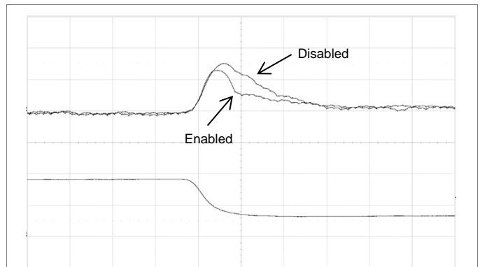
V_I=12\text{ V} , V_O=0.6\text{ V} , C_O = 3 \times 100\ \mu\text{F} + 270\ \mu\text{F}/10\text{m}\Omega , load step 3-9-3 A, 1 A/us. FEEDBACK_EFFORT = 0.8, ZETAP = 1.5. Scale: 20 mV/div, 5 A/div, 10 \mu\text{s} /div.
