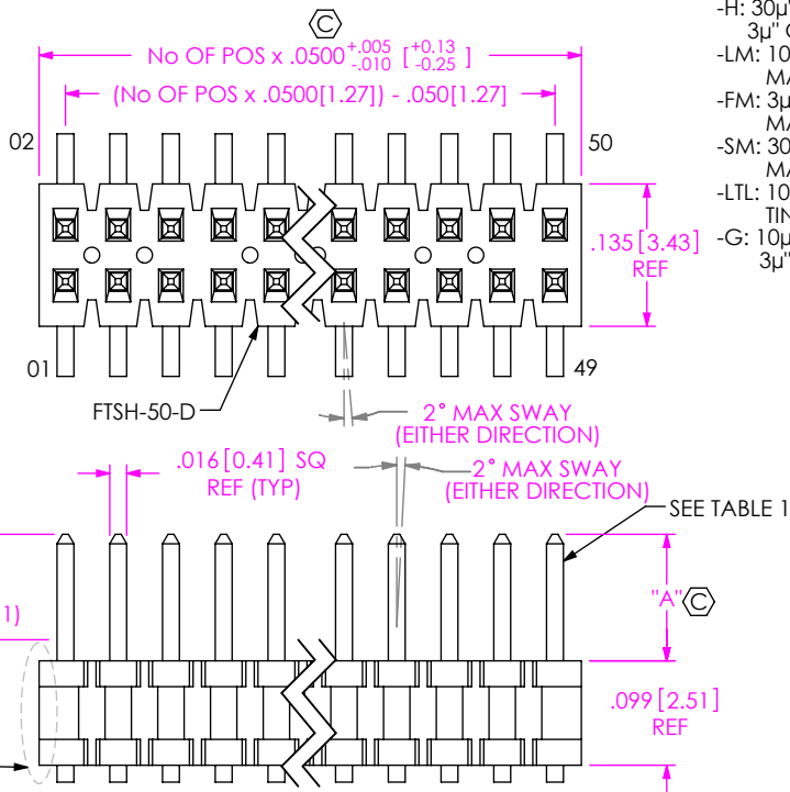
FIG 1 FTSH-1XX-XX-XXX-DV SHOWN
