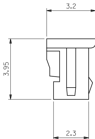
SECT. G-G
