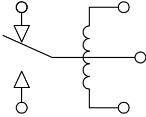
CIRCUIT DIAGRAM (BOTTOM VIEW)
